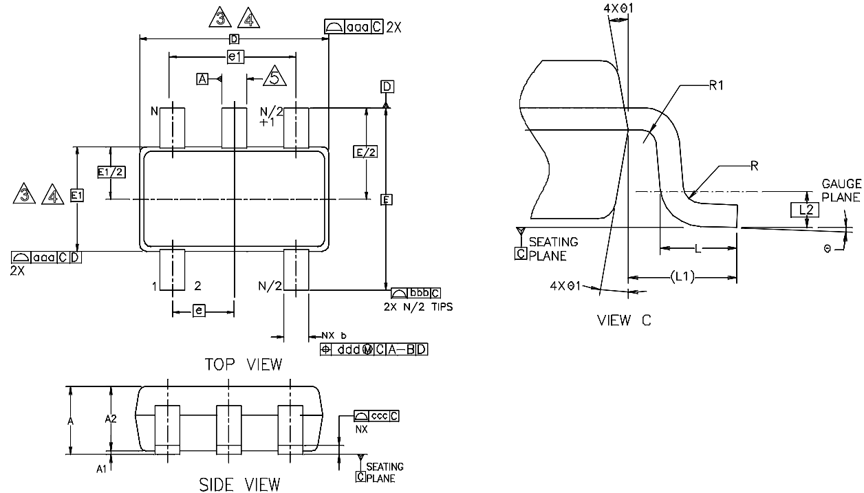
Figure 21. TSOT23-5 Package
